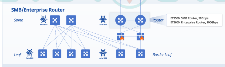
Figure 3: SMB/Enterprise Router
